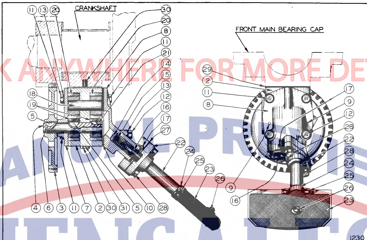
PLATE 5-OIL PUMP
